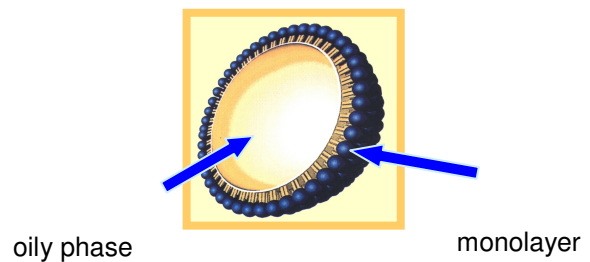
Figure 3 Nanoparticle (model)
