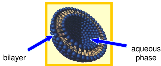
Figure 2: Liposome (model)
